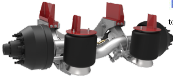
Duramax-UD 20k - Non Steerable
