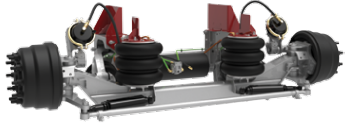
Duralift II 13.5k With Integrated Air - Self Steering
