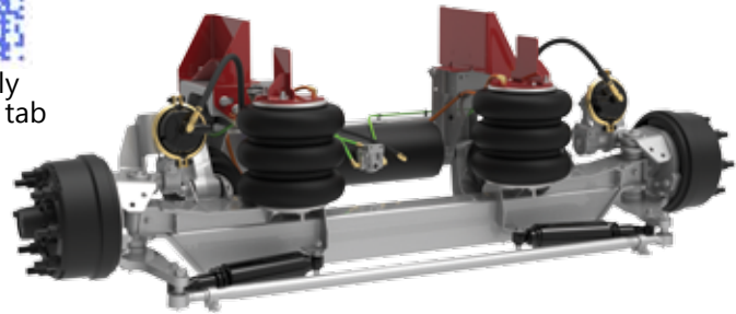
Duralift II 10k With Integrated Air - Self Steering
